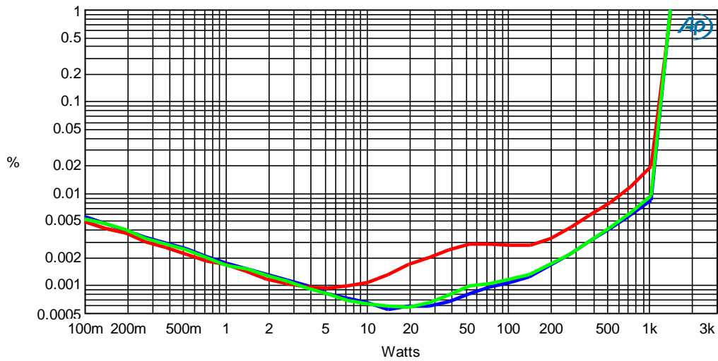
Figure 6: THD+N vs power @ 100 Hz (blue), 1 kHz (green), 6.66 kHz (red), RL = 8 Ohm
