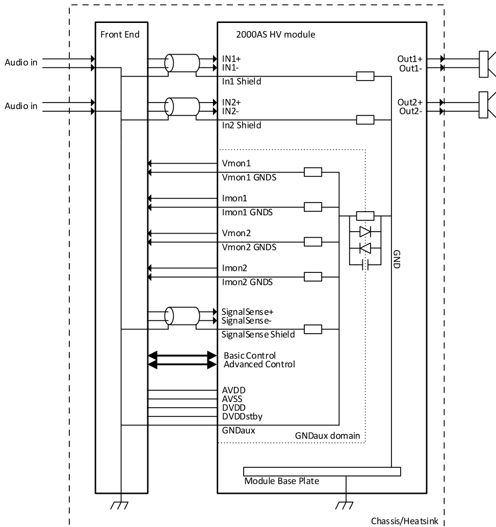
Figure 30: Grounding scheme
