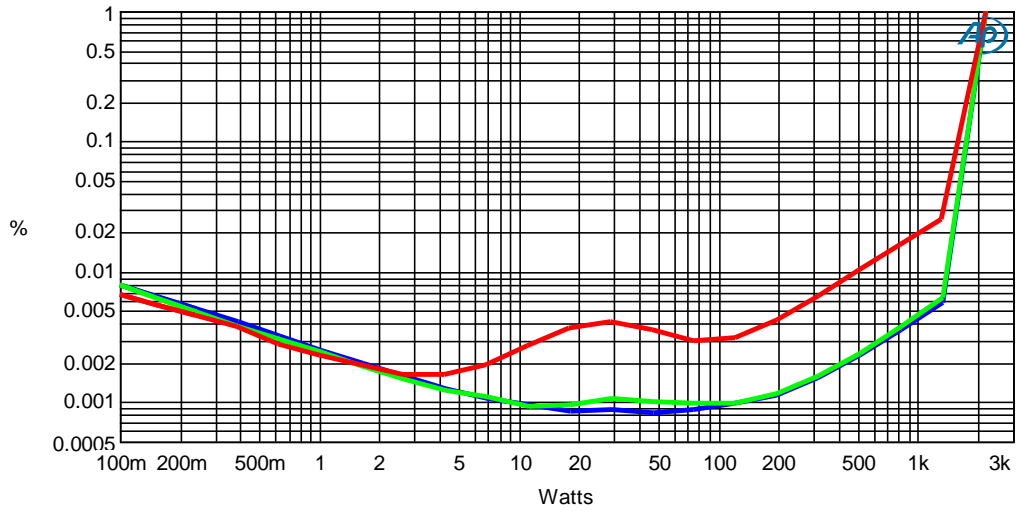
Figure 5: THD+N vs power @ 100 Hz (blue), 1 kHz (green), 6.66 kHz (red), RL = 4 Ohm
