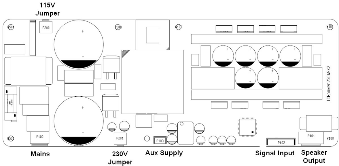
Figure 2: ICEpower250ASX2 connections
