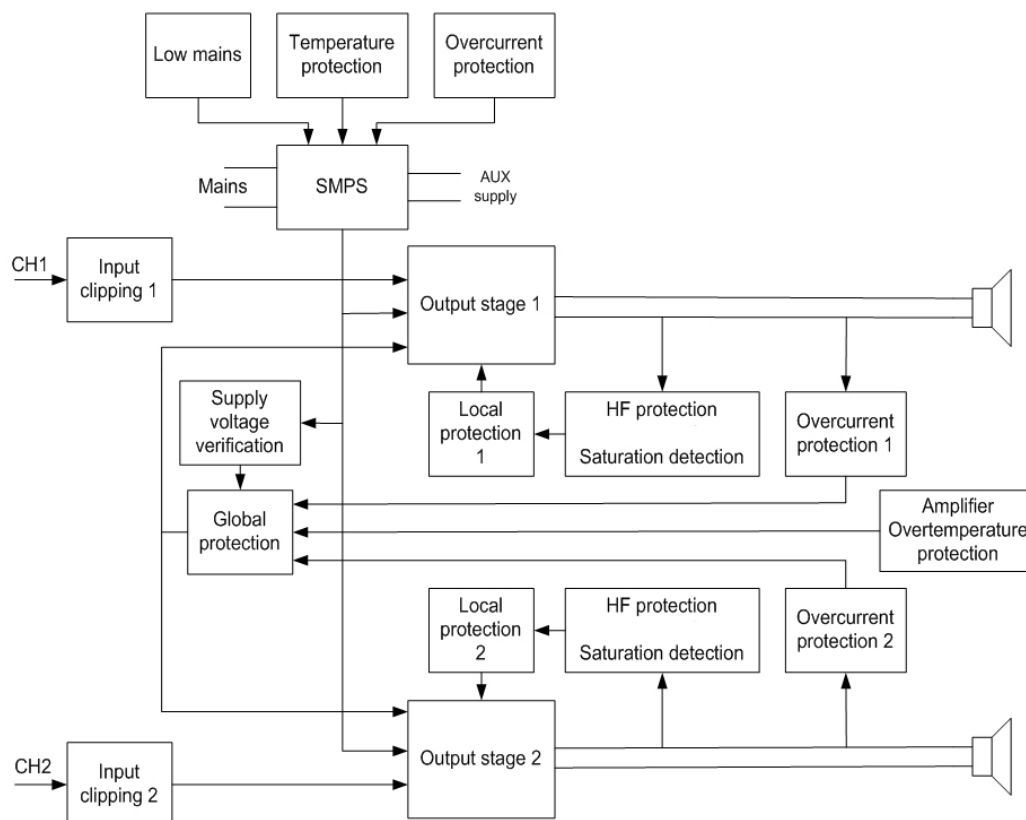
Figure 15: Protection schematic
