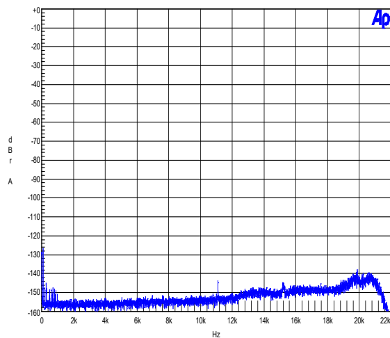
Idle noise (16K FFT). Residual = 80μV(A). (Relative to 250W into 4 ohm)
