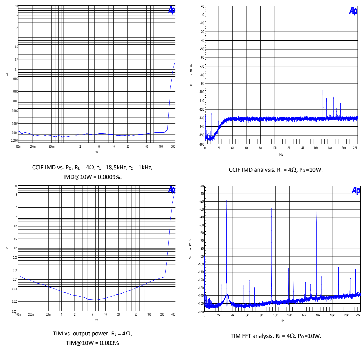
Figure 7: Intermodulation distortion (SE)
