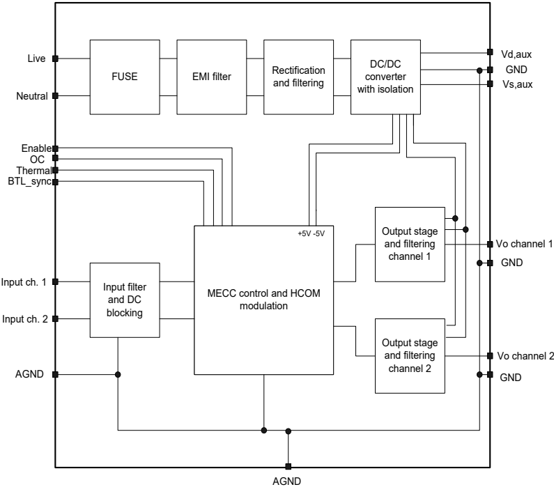
Figure 1: ICEpower250ASX2 block diagram
