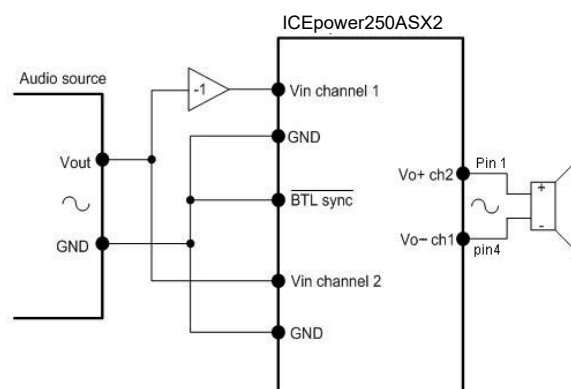
Figure 17: Wiring diagram for the BTL module
