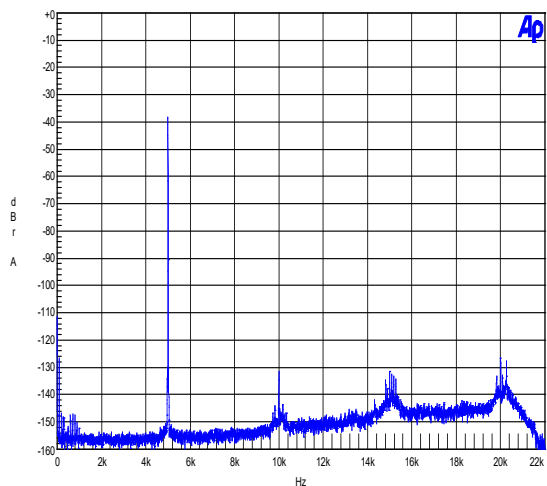
5kHz. Po = 100mW. 4Ω loading. (Relative to 250W into 4 ohm)
