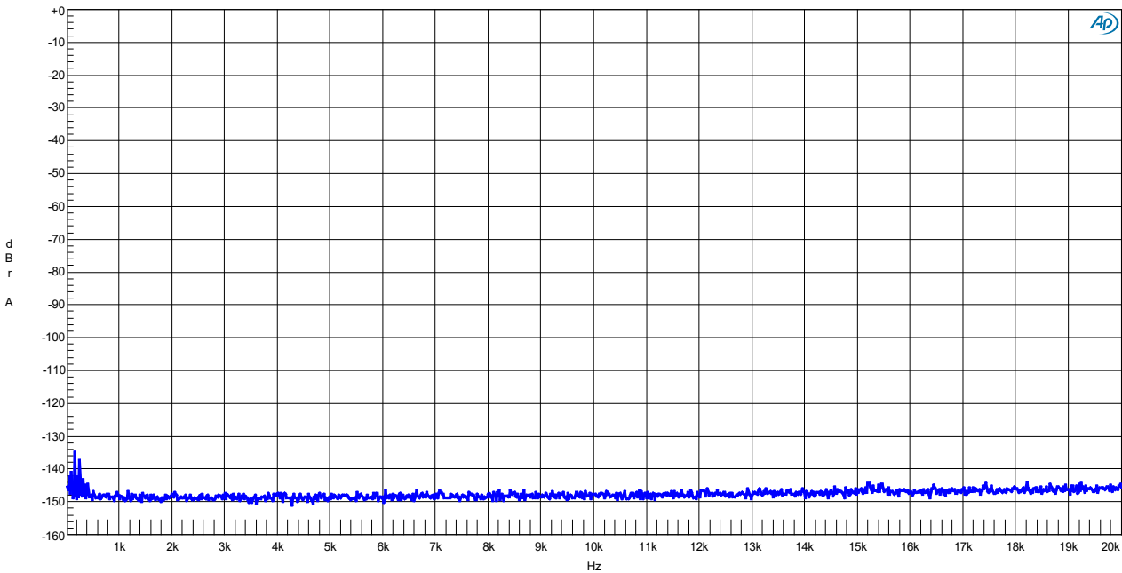
Figure 6: Idle noise (16K FFT). Residual = 75μV(A)
