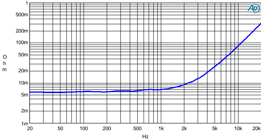
Figure 11: Output impedance at the output terminals
