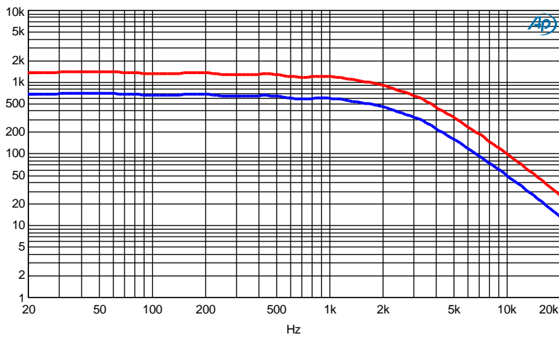
Figure 12: Damping factor vs. frequency 4 Ω (blue) and 8 Ω (red)
