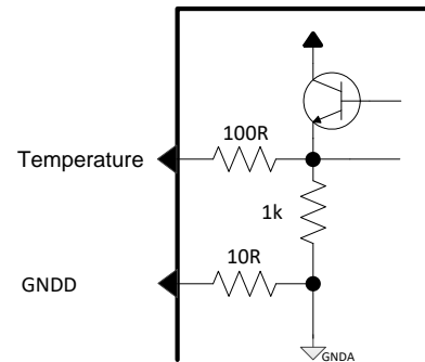
Figure 19: Temperature monitor pin interface.
