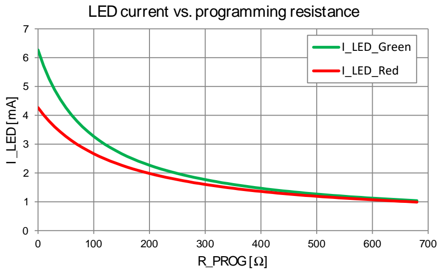
Figure 24: LED intensity/current programming
