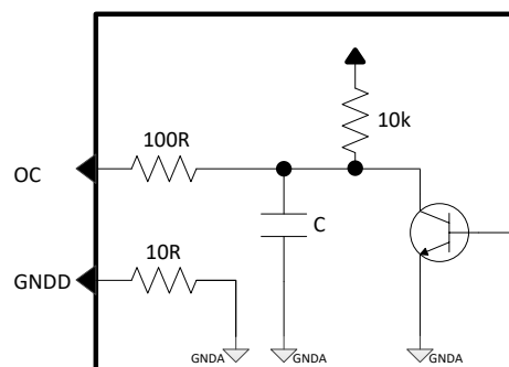
Figure 17: Over current monitor pin
