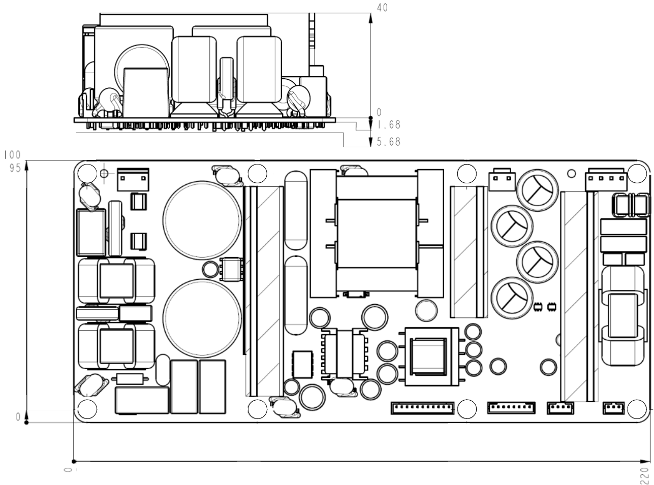
Figure 3: Outer dimensions ICEpower700AS1
