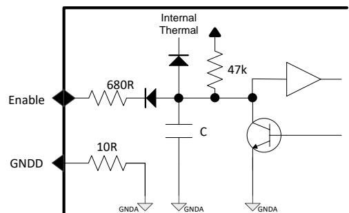
Figure 20: Amplifier enable pin interface.
