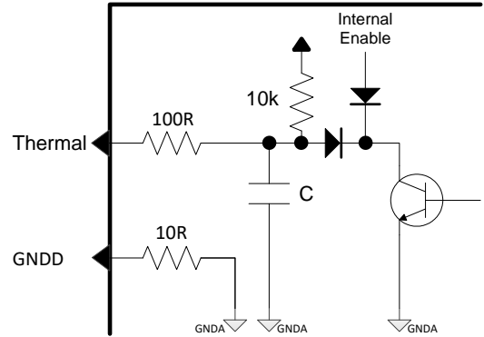
Figure18: Thermal protection pin interface.
