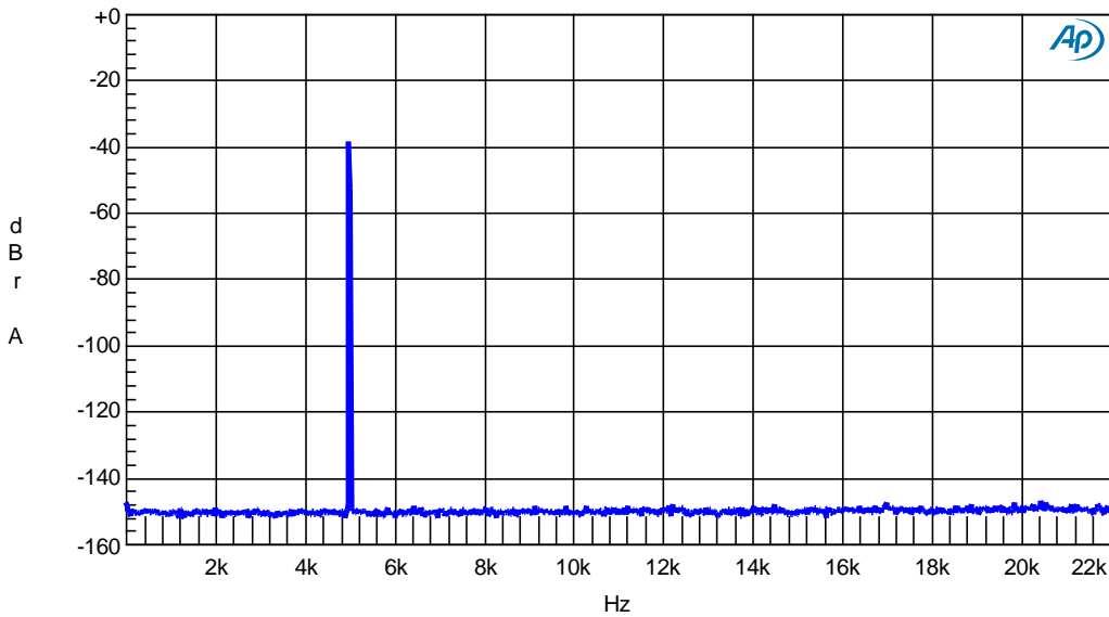
Figure 8: f = 5 kHz. Po = 100 mW, RL = 4 \Omega (Relative to 700 W into 4 \Omega )
