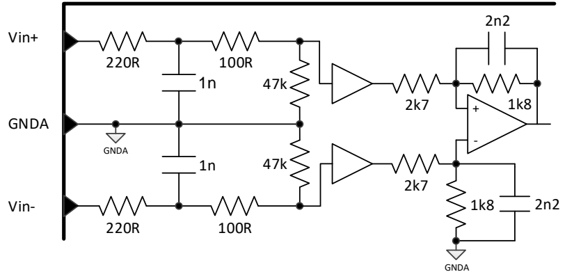
Figure 15: Balanced input buffer
