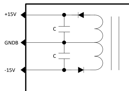
Figure 21: +/-15 V auxiliary supply
