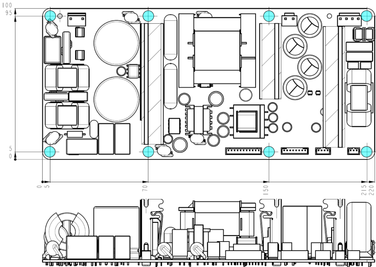
Figure 33: Mounting by bottom side spacers
