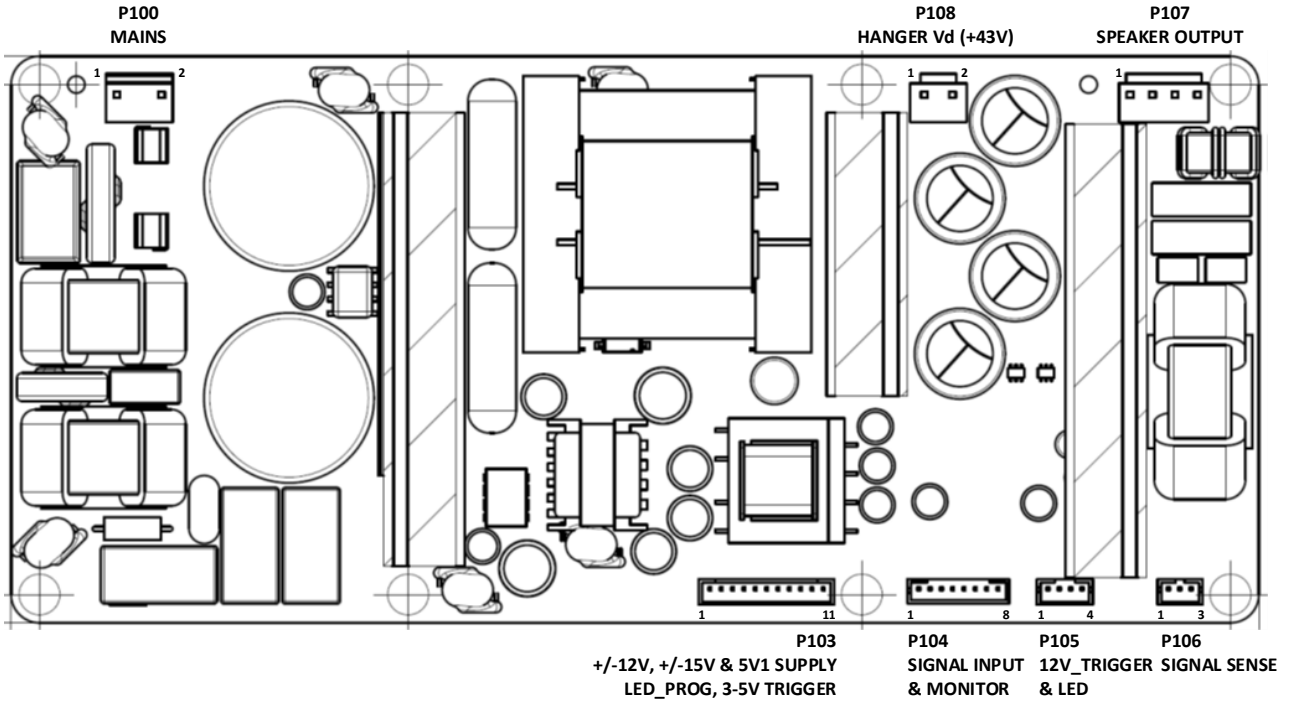
Figure 2: ICEpower700AS1 connectors overview
