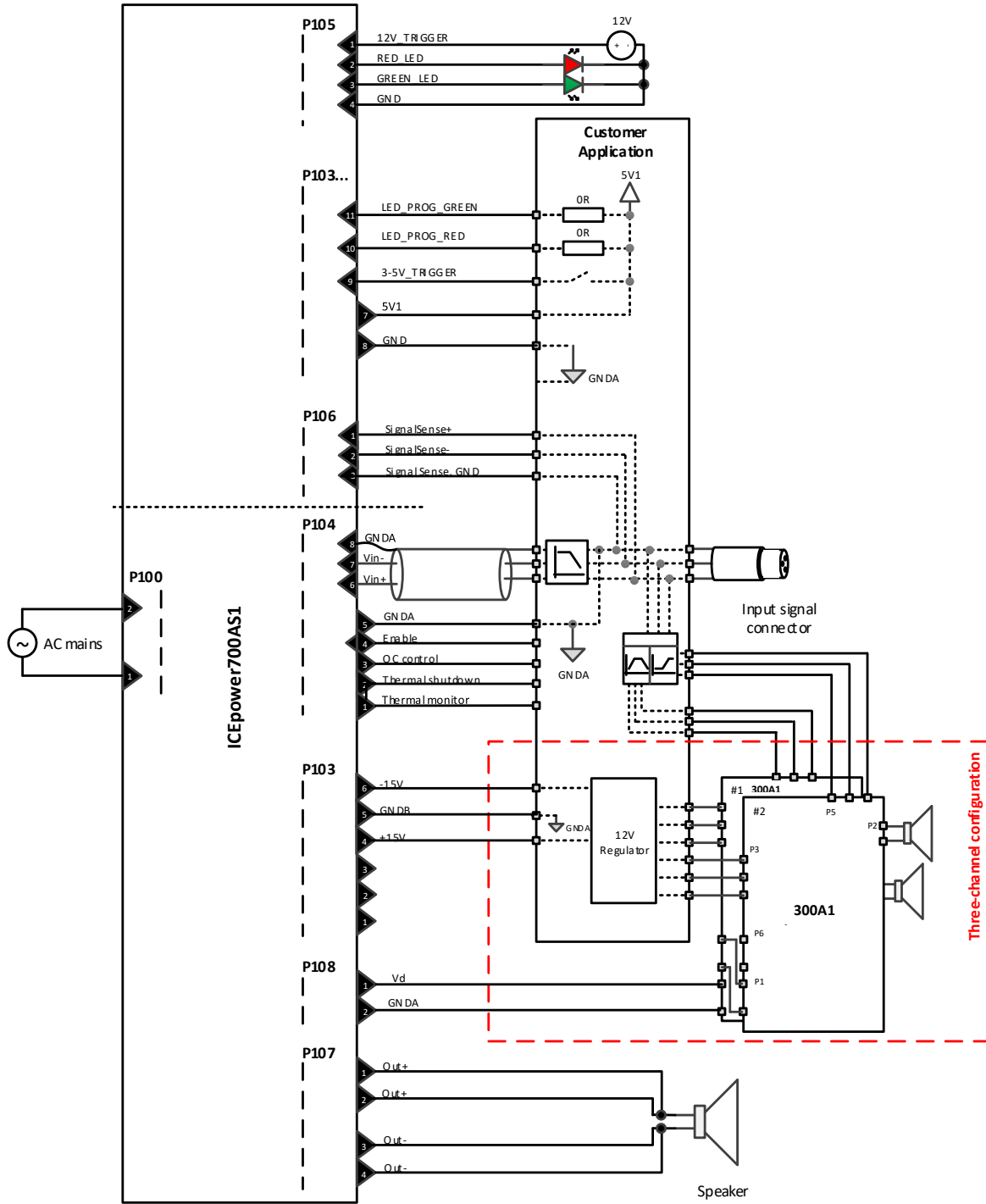
Figure 30: Three channel configuration, Balanced audio input
