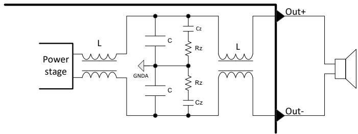
Figure 16: Output filter section with compensating Zobel network
