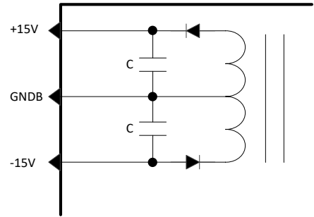
Figure 27: +/-15 V auxiliary supply
