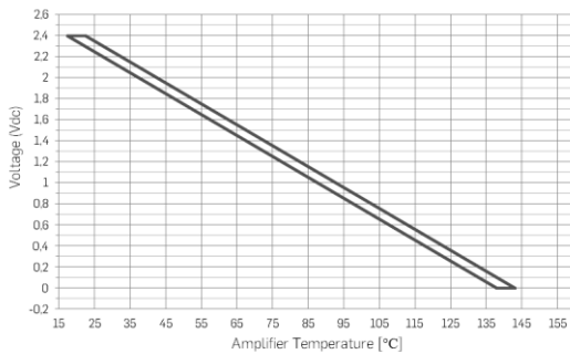
Figure 24: ICEpower700AS2 Temperature Monitor.
