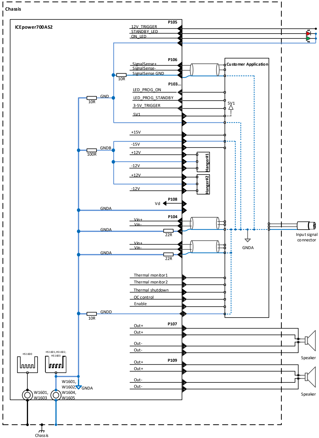
Figure 36: ICEpower700AS2 grounding scheme
