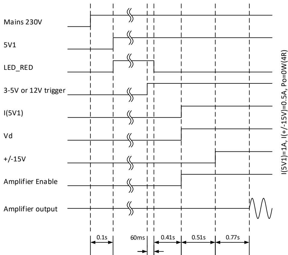
Figure 31: Power up from Mains on and trigger high, typical timing at 25 °C ambient.
