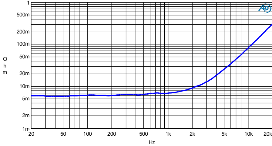
Figure 16: Output impedance at the output terminals
