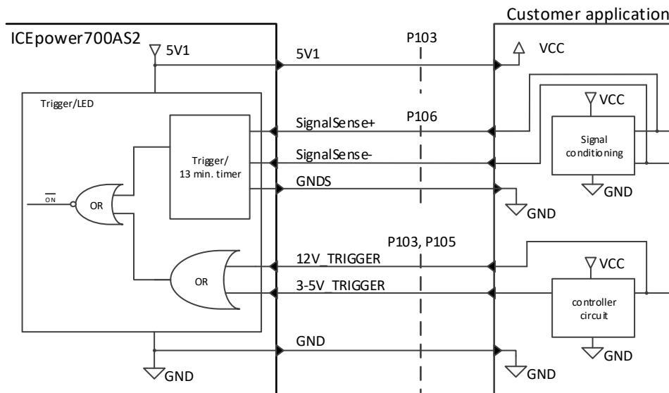
Figure 28: ICEpower700AS2 Trigger and Signal Sense connection scheme
