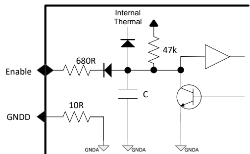
Figure 26: Amplifier enable pin interface.
