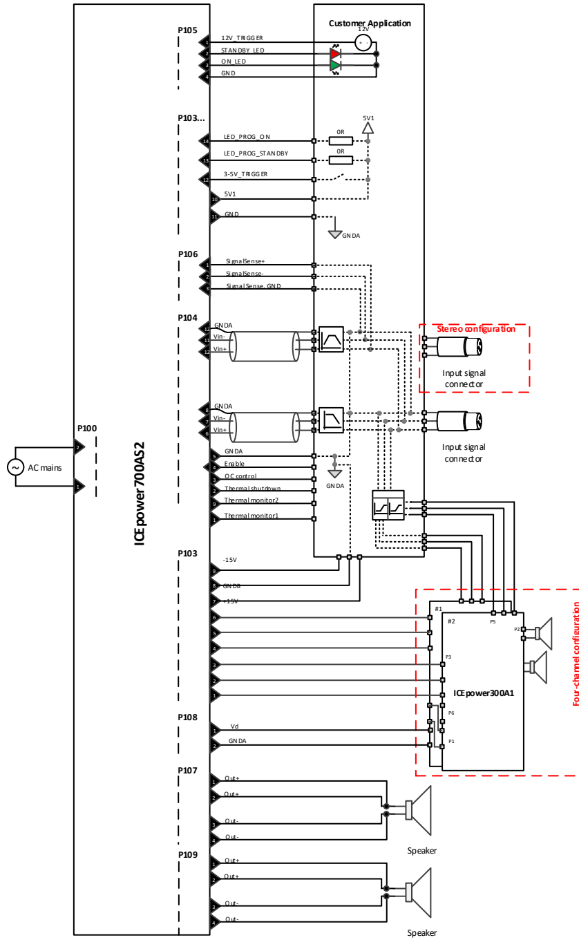
Figure 35: Four channel configuration, Balanced audio input
