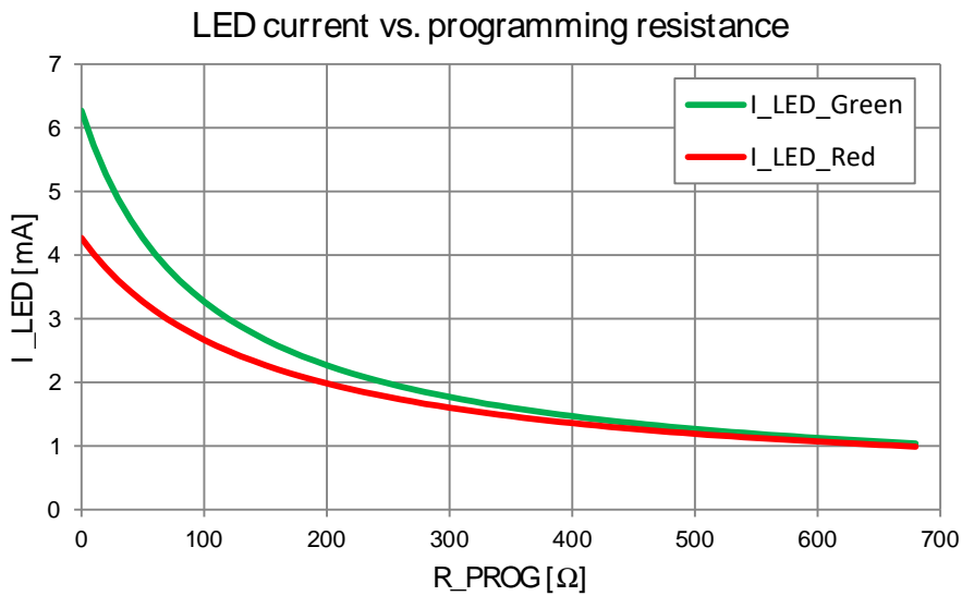
Figure 30: LED intensity/current programming
