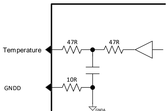
Figure 25: Temperature monitor pin interface.
