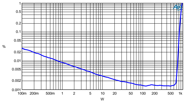
Figure 14: TIM(DIM30) vs. Po, RL=4 Ω 2)
