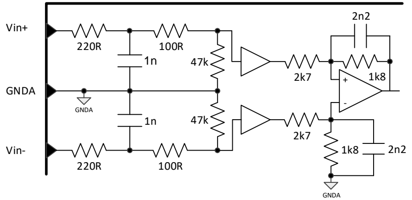
Figure 20: Balanced input buffer.
