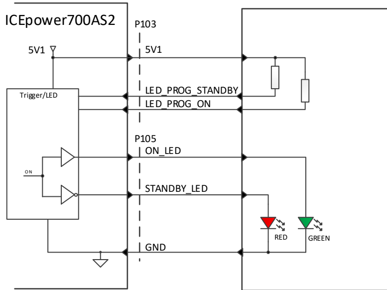
Figure 29: Application of the current programmable LED driver
