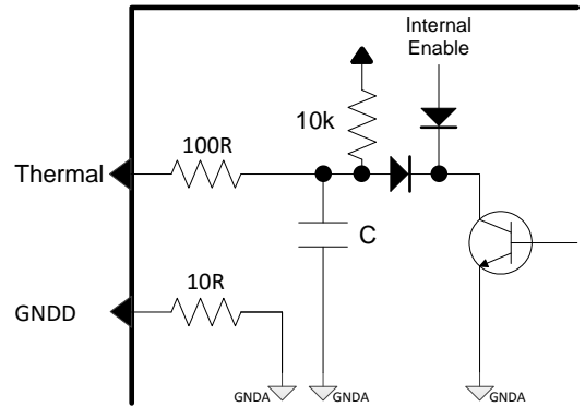
Figure 23: Thermal protection pin interface.
