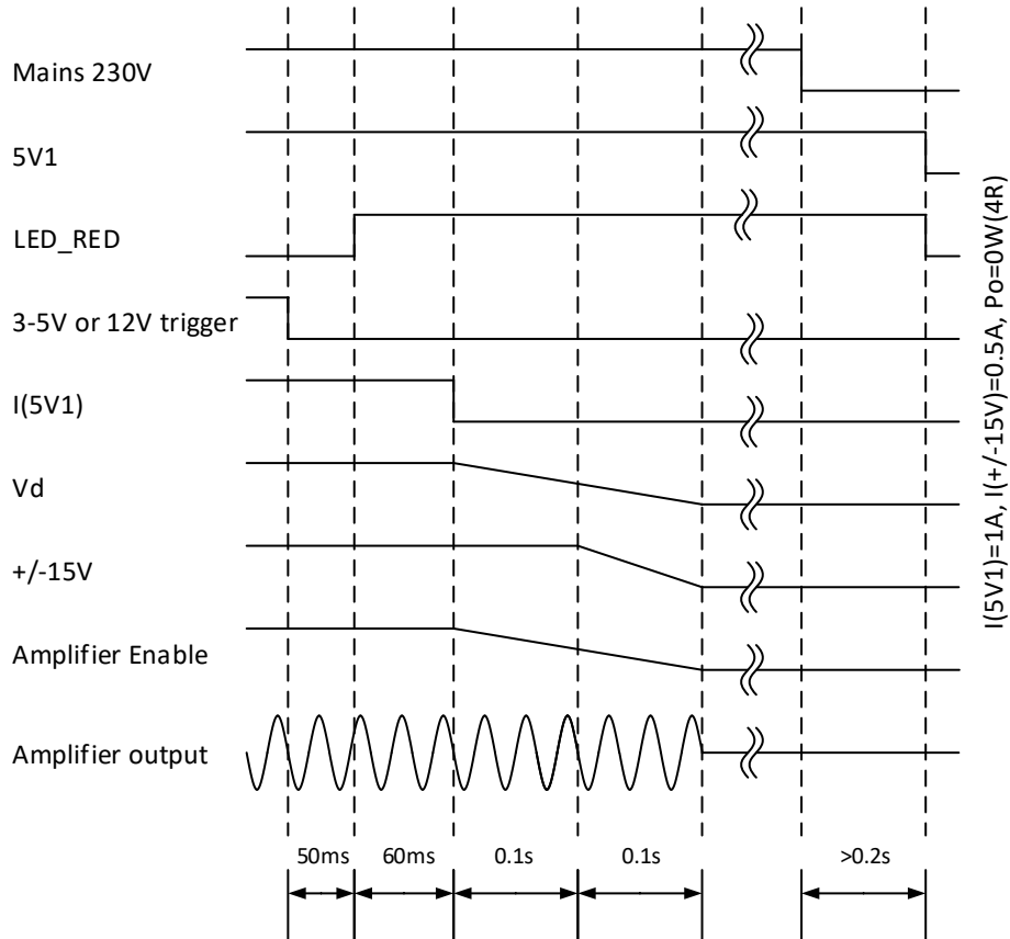
Figure 32: Power down from trigger low and Mains off, typical timing at 25 °C ambient.
