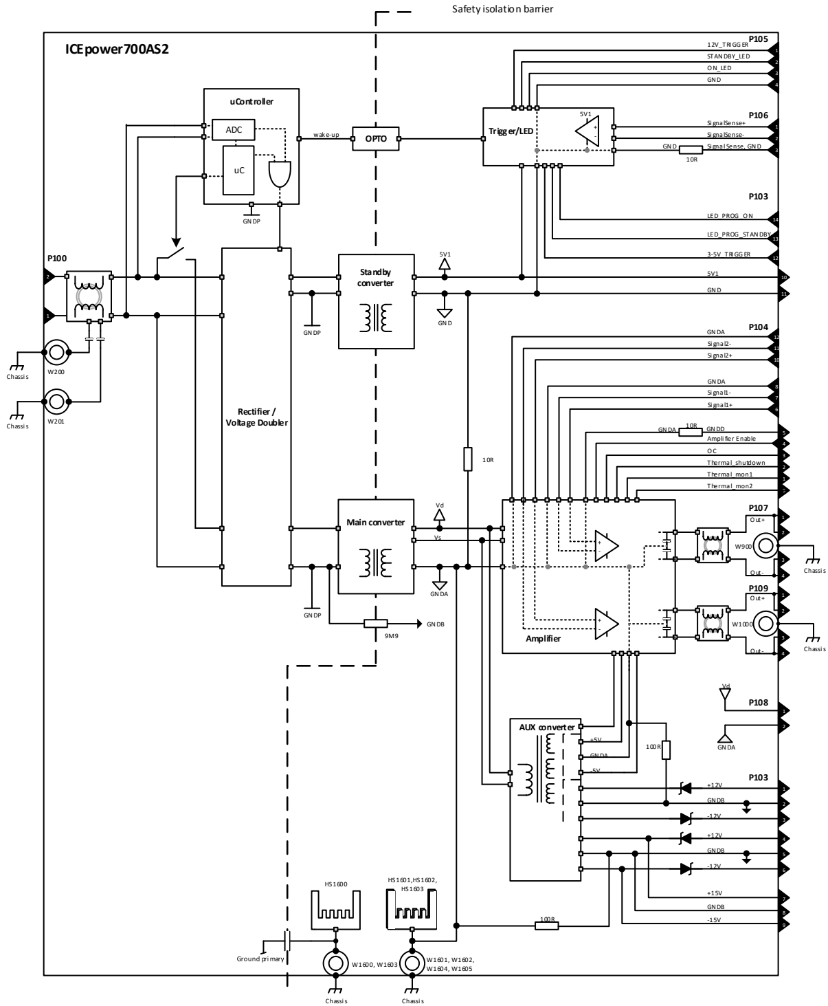
Figure 1: ICEpower700AS2 block diagram
