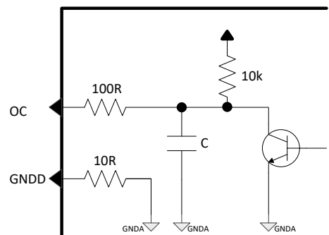
Figure 22: Over current monitor pin interface.
