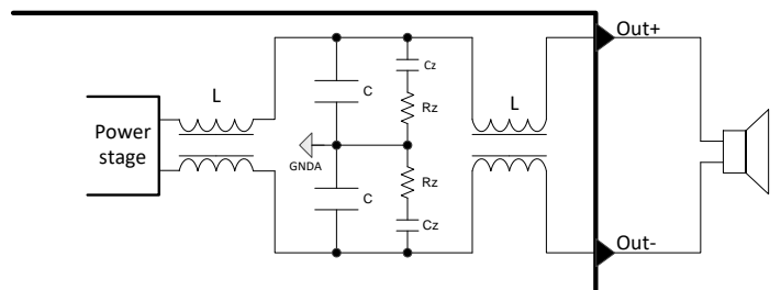
Figure 21: Output filter section with compensating Zobel network.
