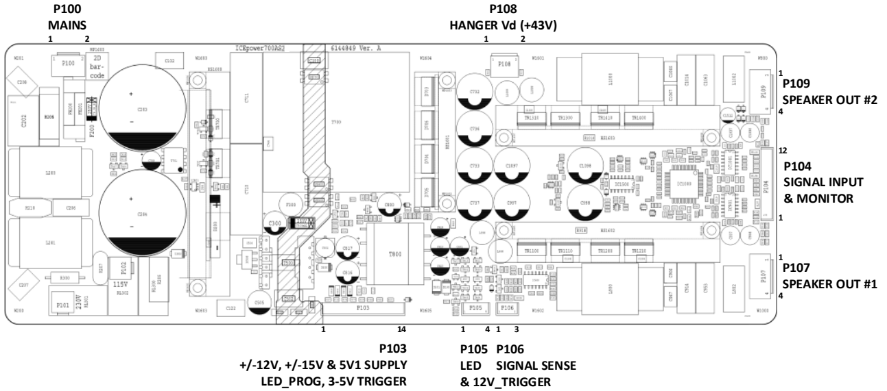
Figure 2: ICEpower700AS2 connector overview
